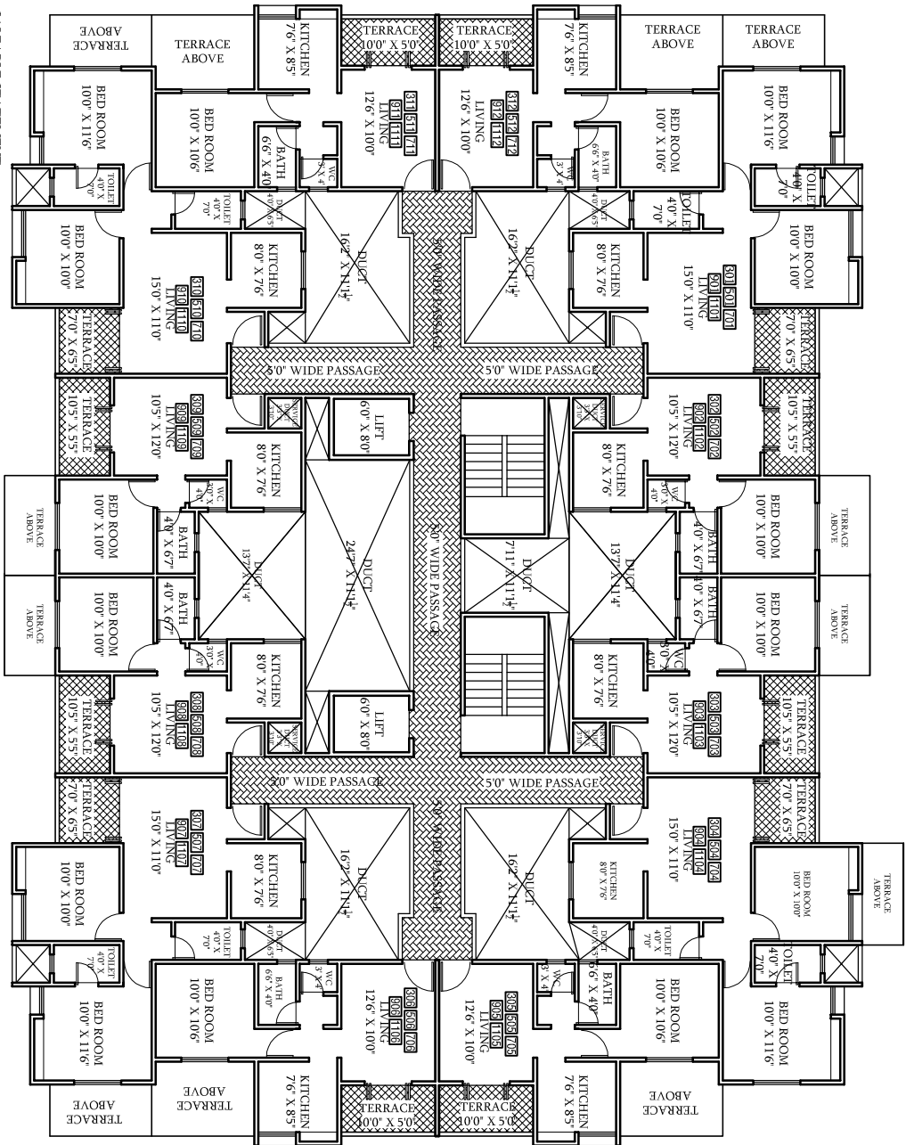
TYPICAL FLOOR PLAN (3rd, 5th, 7th, 9th & 11th)
